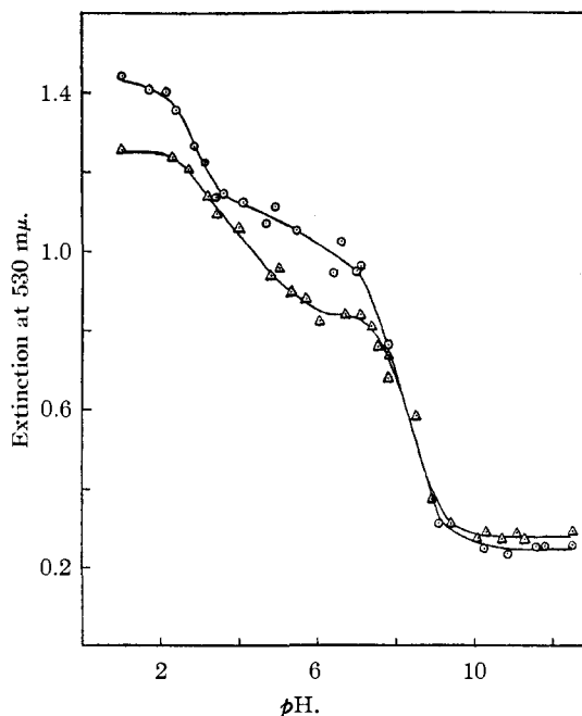
Fig. 1.—Structure changes with changing pH: ○, 7- o -tolylazo-8-quinolinol-5-sulfonic acid; Δ, 7- o -tolylazo-8-hydroxyquin-aldine-5-sulfonic acid.
